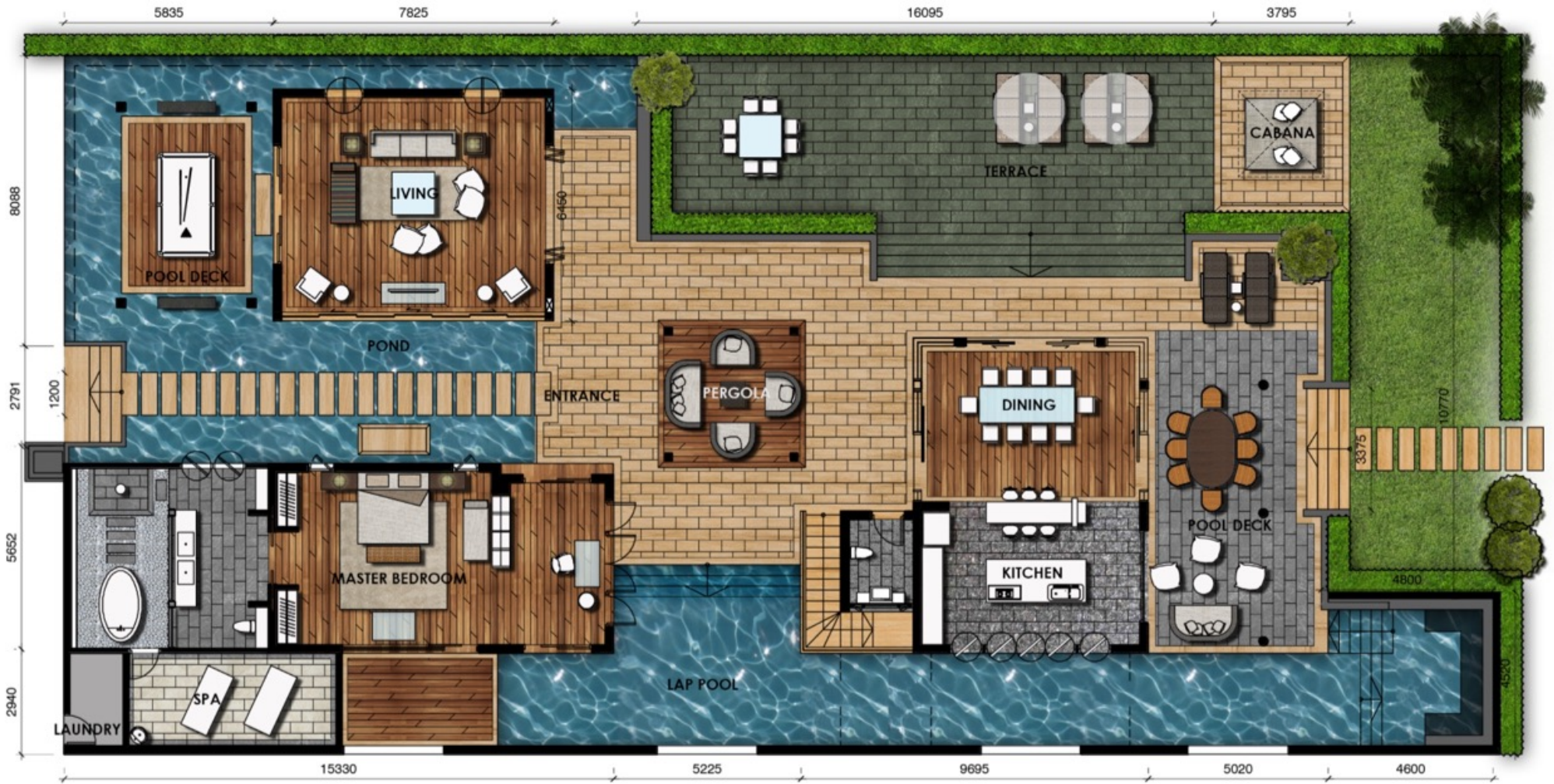
MAIN VILLA LAYOUT GROUND FLOOR
